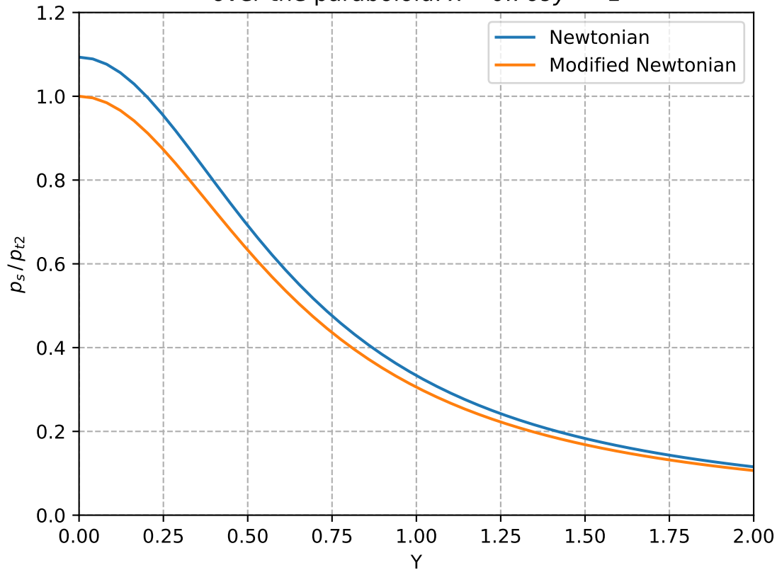
Surface-pressure distribution over the paraboloid: x = 0.769y^2 - 1
